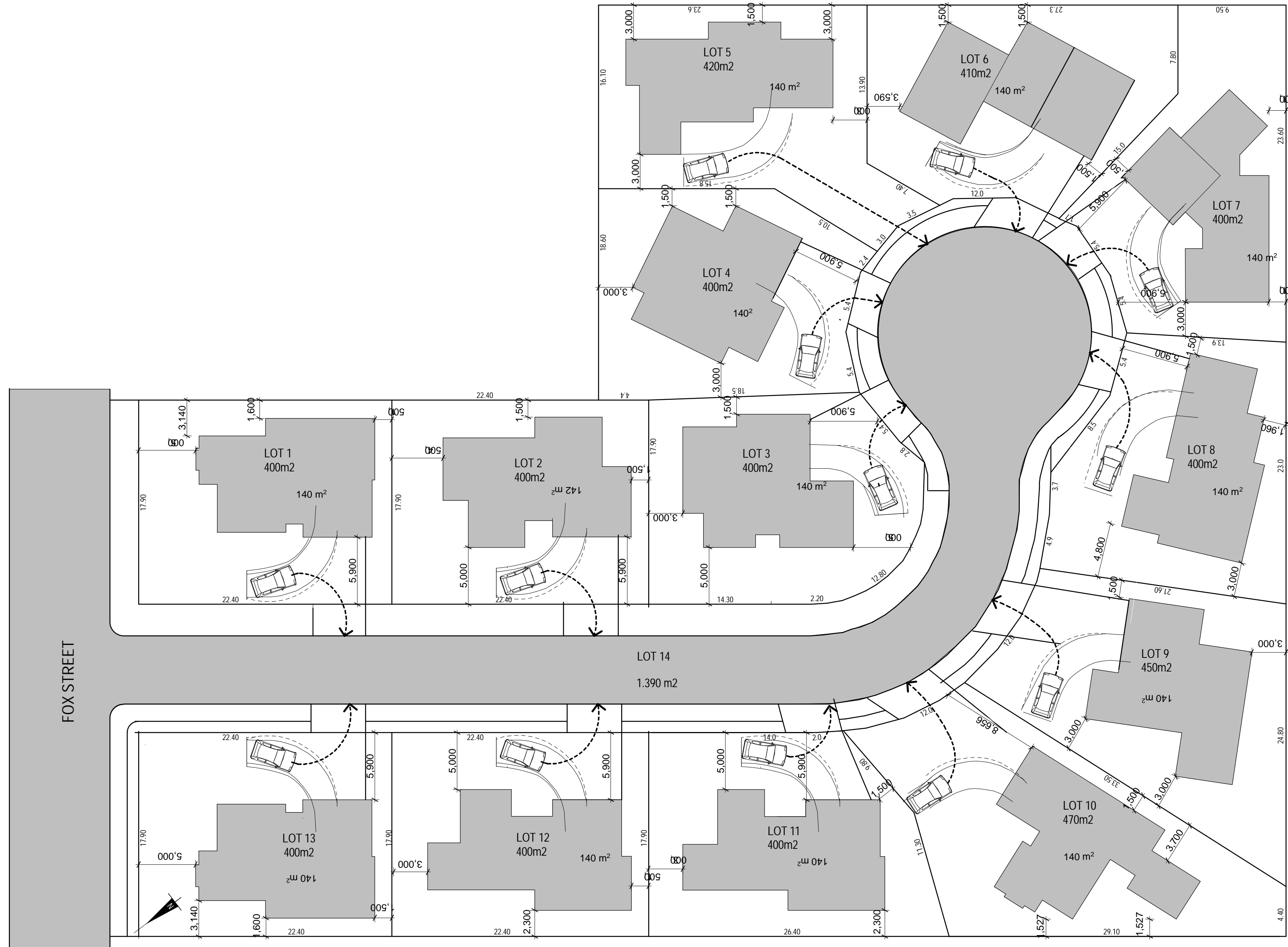
PROPOSED LAYOUT Scale 1:250
